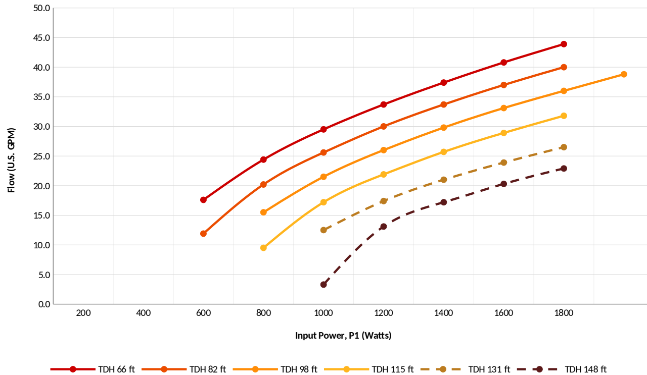
HS-35-115 Performance Curve
