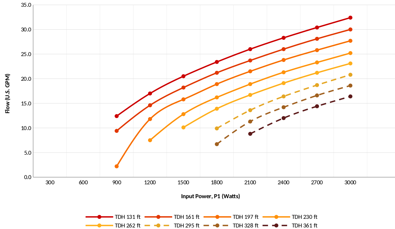
HS-22-308 Performance Curve
