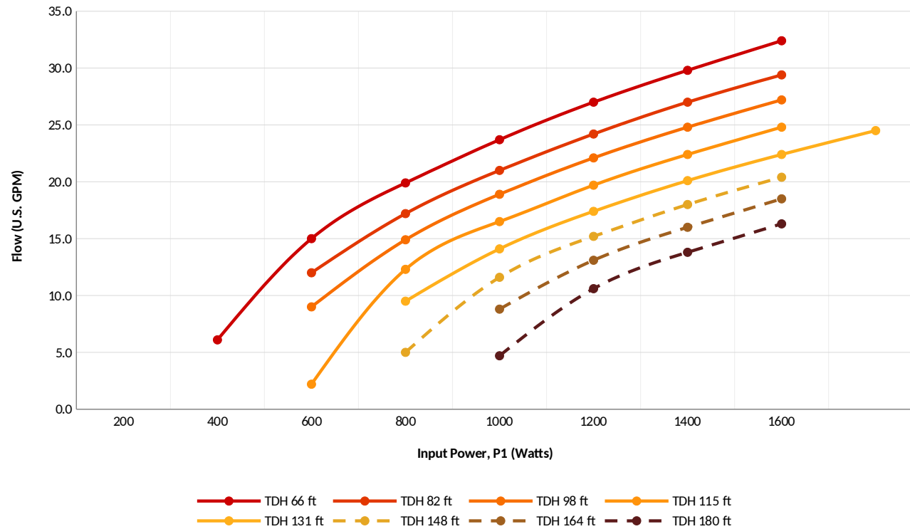
HS-22-154 Performance Curve
