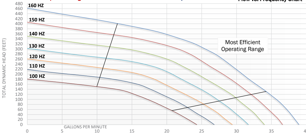
SunPumps Centrifugal Submersible Model HS 35-115 AC/DC R1
