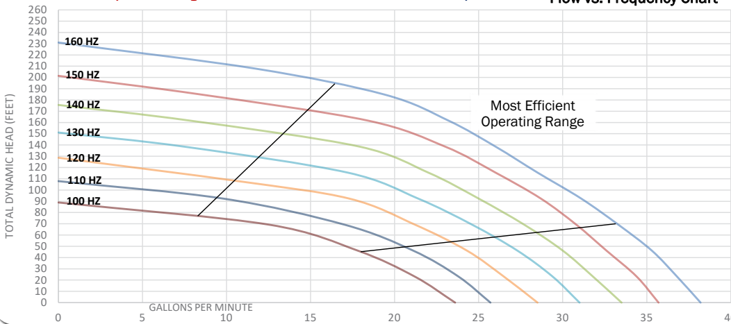
SunPumps Centrifugal Submersible Model HS 22-308 AC/DC
