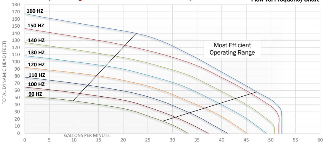
SunPumps Centrifugal Submersible Model HS 35-190 AC/DC
