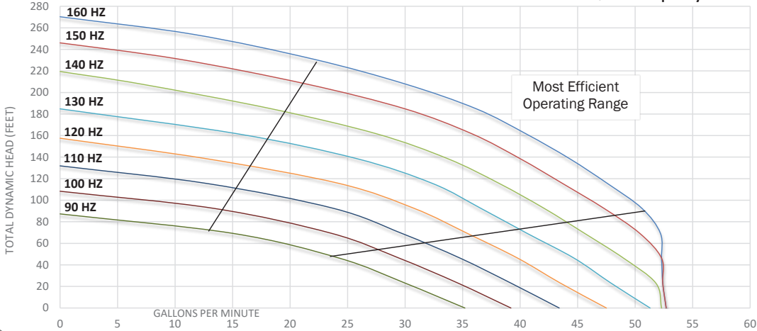
SunPumps Centrifugal Submersible Model HS 35-190 AC/DC
