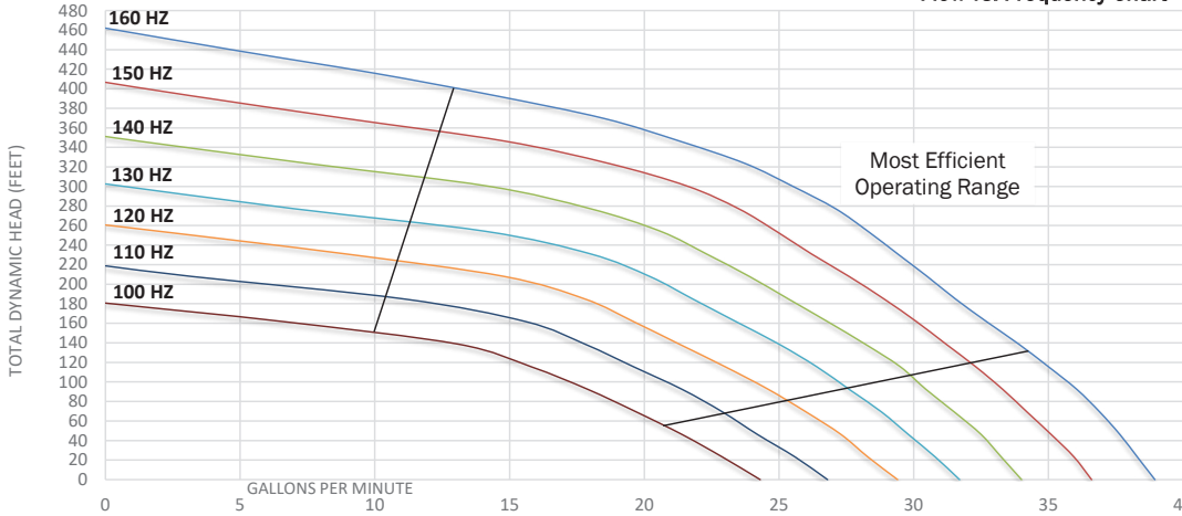
SunPumps Centrifugal Submersible Model HS 22-308 AC/DC
